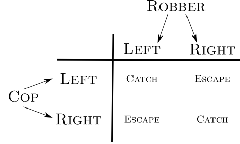
Figure 1: Cop and robber
