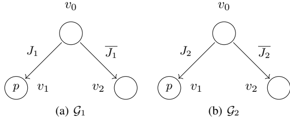
Figure 2: Games \mathcal{G}_1 and \mathcal{G}_2
