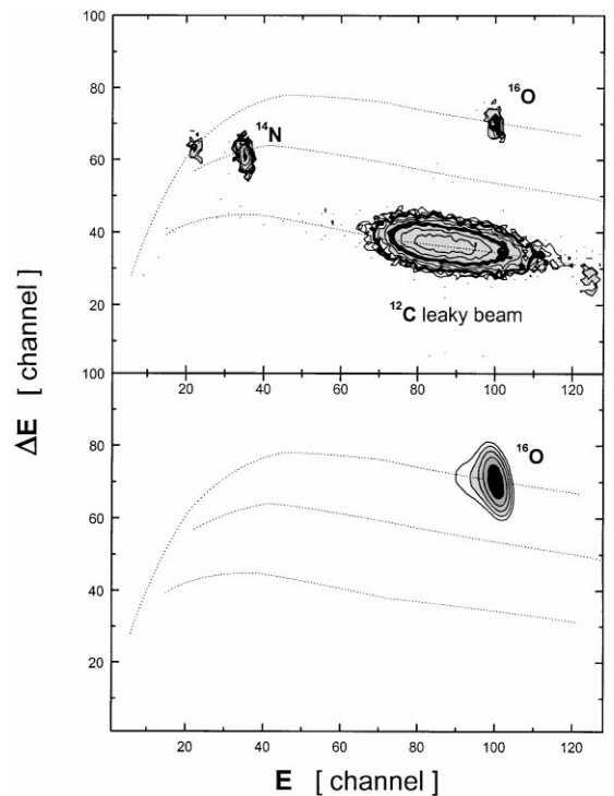
Fig. 5. The \Delta E - E identification matrix for a ^{12}\text{C}^{3+} ion beam of 14 MeV is shown with the injection magnet (Fig. 1) set at mass 12 (upper part) and at mass 16 (lower part): the contaminant ^{16}\text{O} beam appears at the same point in the matrix. Also visible in the upper part is a contaminant ^{14}\text{N} beam arising from the nitrogen stripper gas. The peak far to the left represents another contaminant ^{16}\text{O} beam with a 2^+ charge state. The dotted curves correspond to the expected locations of these ions in the matrix.
