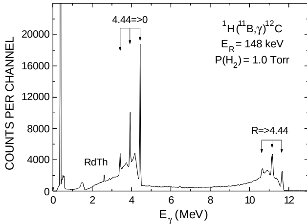
Fig. 7. Summed spectrum of the 6 Ge detectors obtained at the E_R = 148 keV resonance of ^1\text{H}(^{11}\text{B}, \gamma)^{12}\text{C} , which emits predominantly the cascade transitions with energies E_\gamma = 4.44 and 11.67 MeV.
