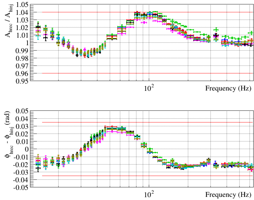
Figure 5. Transfer function between the reconstructed h(t) signal ( h_{\text{rec}} ) and the injected signals on NE mirror ( h_{\text{inj}} ). The different colors correspond to various sets of injections during the O2 run. The comparison of h_{\text{rec}} and h_{\text{inj}} is within \pm 4\% in amplitude and \pm 35 mrad in phase as shown by the red lines.
