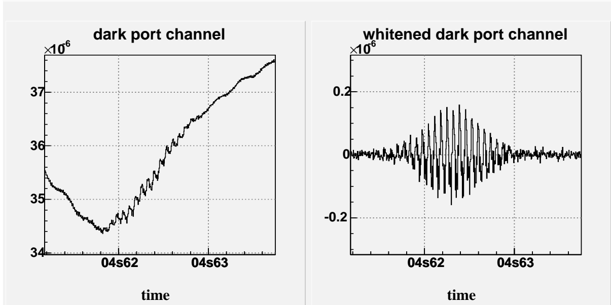
FIG. 5: Time series in the dark port channel (left) and the whitened dark port channel (right) of the loudest event detected by the EGC pipeline in the search for GW bursts in the C7 data. This event was seen with a SNR of 69.7 at a frequency about 1466 Hz.
