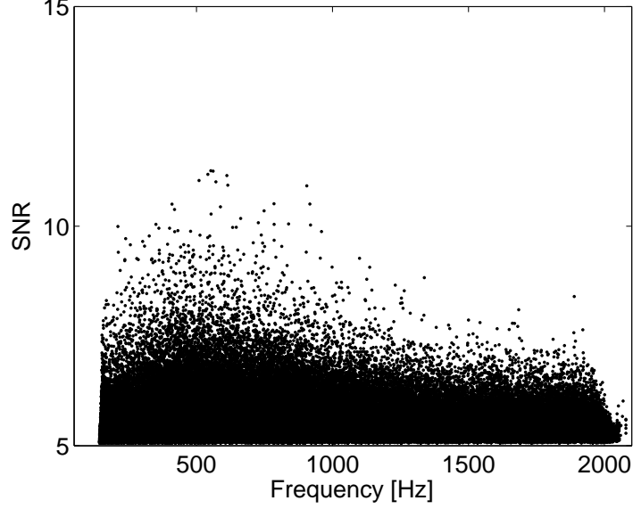
FIG. 8: SNR as a function of the frequency of the triggers obtained on the GW strain amplitude channel by EGC after applying all vetoes on the full C7 data set. The distribution around 2 kHz is due to the templates' placement; some Sine Gaussian templates have a central frequency which can slightly exceed 2kHz.
