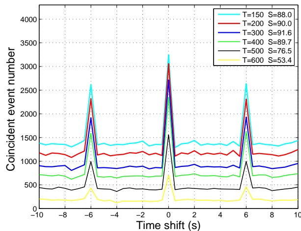
FIG. 4: Number of coincident triggers between the GW strain amplitude and the auxiliary channel that has been used to define the Seismic veto, as a function of the time shift introduced in the Seismic veto list. The different curves have been obtained for different threshold values (T). S is the significance. The peaks correspond to the stepping motor that have been activated each 6 seconds during the playground dataset. The different curves have been obtained for various values of the threshold applied on the auxiliary channel RMS. The maximal value of the significance is obtained for a threshold of T=300.
