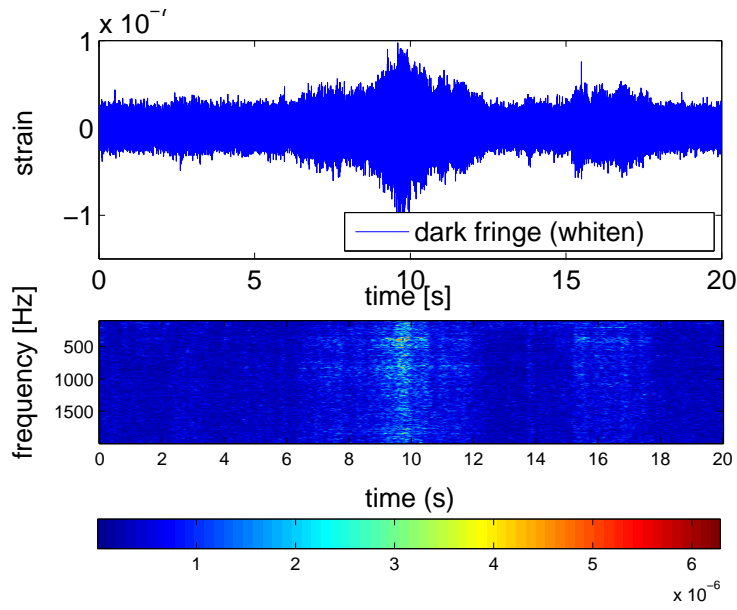
FIG. 2: An example of a Burst of Bursts (BoB) around t \simeq 10 s. The upper plot shows the whitened interferometer dark port channel amplitude as a function of time, while the bottom plot is the corresponding spectrogram.
