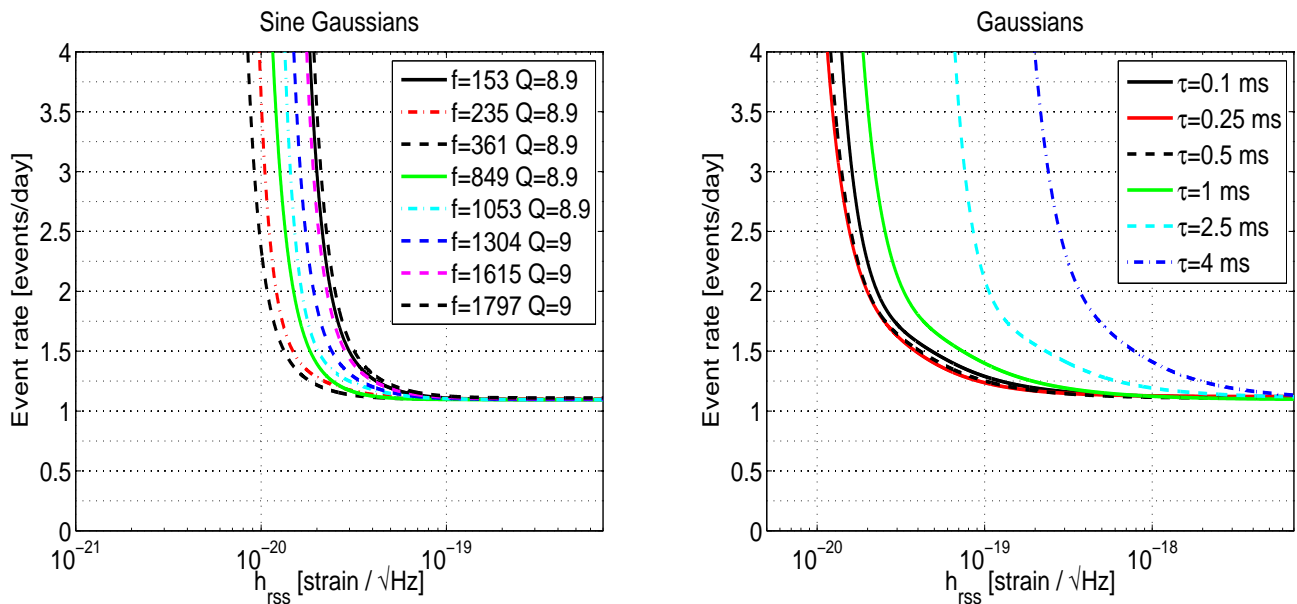
FIG. 12: Event rate as a function of the h_{rss} exclusion plots at 90% confidence level obtained in the Virgo C7 data. The left plot corresponds to GW burst events that can be modeled by a Sine Gaussian with a Q of 8.9 or 9 for frequencies, f , covering the most promising part of the C7 frequency range. The right plot corresponds to GW burst events that can be modeled by a peak of different widths, \tau , from 0.1 ms up to 4 ms.
