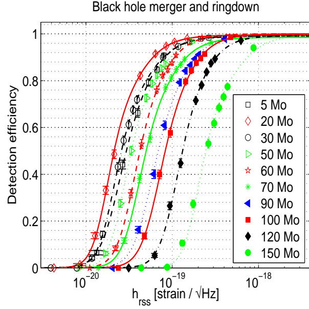
FIG. 11: Detection efficiencies from the search analysis as a function of the signal strength h_{rss} for the BBH merger and ringdown waveforms for different BH total masses (but where the two individual component masses are equal). The efficiencies were computed for random polarization, inclination angles, and sky positions. The error bars take into account only the statistical error on the detection efficiency.
