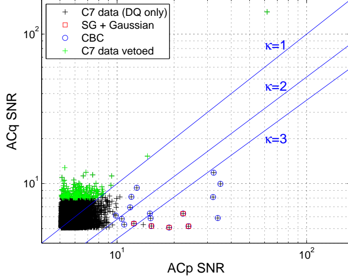
FIG. 6: SNR of the coincident EGC triggers in the two quadrature demodulated channels of the output dark port signal: ACp (in phase) and ACq (in quadrature). The time coincidence window of the triggers seen in the two channels is 10 ms. The Seismic, SSFS, B2 and 1111Hz vetoes have already been applied. The peculiar event appears very isolated with respect to the other triggers with its ACq SNR of 141. The hardware injection signals, which were seen in both of the two demodulation phase channels, are indicated by the circles for burst-like signals and by the squares for the compact binary coalescence (CBC) signals.
