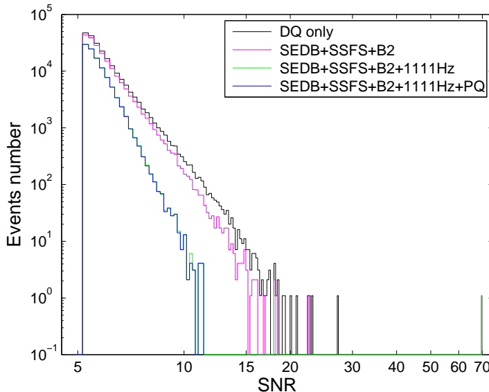
FIG. 7: SNR distribution of the triggers obtained on the GW strain amplitude channel by EGC after applying all vetoes on the full C7 data set.
