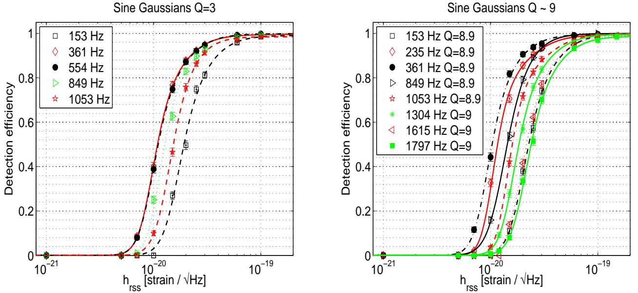
FIG. 10: Detection efficiency of the search analysis as a function of the signal strength h_{rss} at Earth for Sine Gaussian waveforms with different central frequencies f_0 and for two different values of the Q_0 factor: left Q_0 = 3 , right Q_0 \sim 9 . The efficiencies were computed for sources at random sky locations. The error bars take into account only the statistical error on the detection efficiency.
