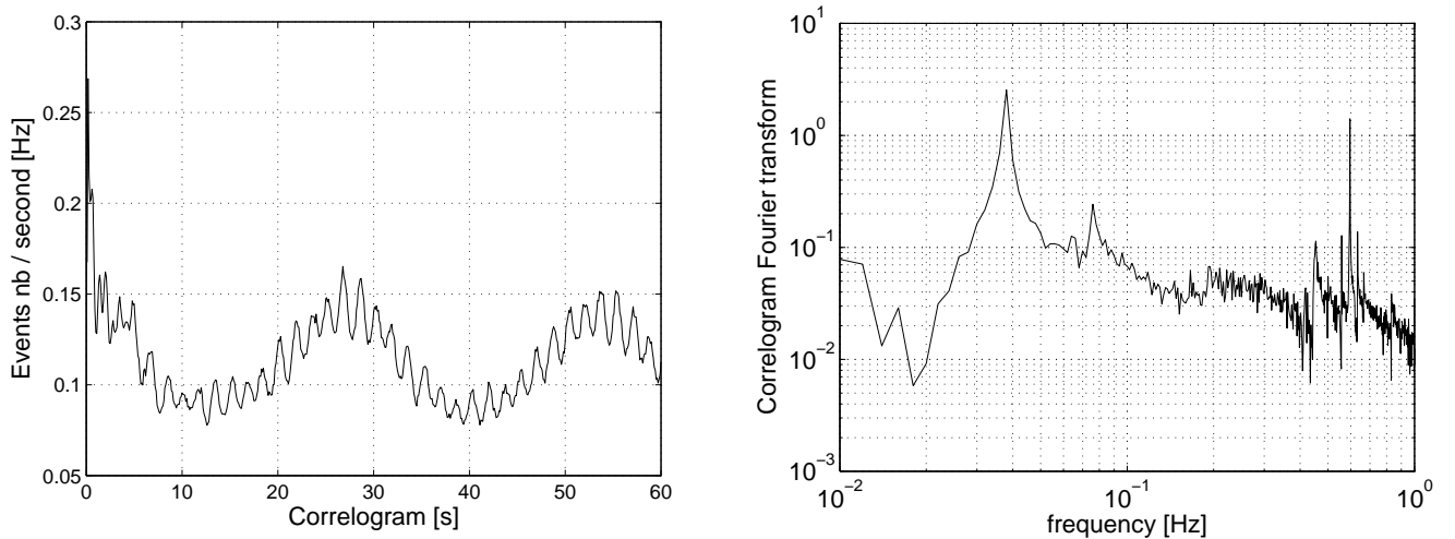
FIG. 3: Left: the correlogram of the triggers found by the EGC pipeline in the C7 dataset. A peak around T \simeq 27 s is present, with a replica at 54 s. A 0.6 Hz modulation is also visible, and this frequency corresponds to the pendulum mode of the last stage of the Virgo suspension. Right: the Fourier transform of the correlogram. The 37 mHz mechanical resonance between the two last stages of the Virgo suspension is clearly visible.
