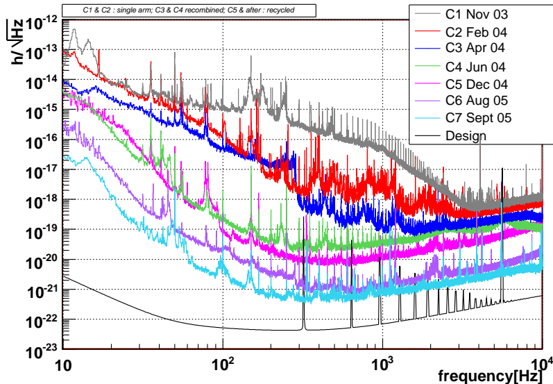
FIG. 1: Sensitivity curves obtained between 2003 and 2005 during the commissioning of the Virgo detector before the 2005 shutdown. The black curve is the Virgo nominal sensitivity curve which has been computed assuming a 10 W laser.
