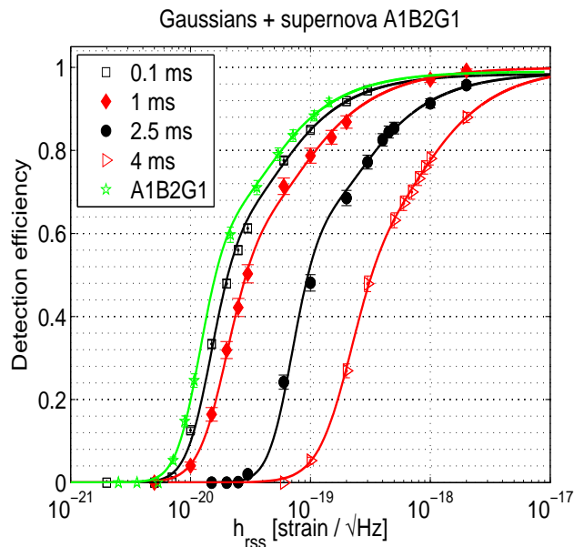
FIG. 9: Detection efficiency of the search analysis as a function of the signal strength h_{rss} at Earth for the Gaussian waveforms (with \tau specified in the legend) and one core collapse simulated waveform (A1B2G1). The efficiencies were computed for sources at random sky locations. The error bars take into account only the statistical error on the detection efficiency.
