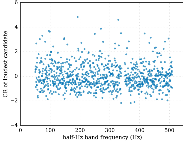
FIG. 5. Highest values of the significance (CR) in every half-Hz band as a function of band frequency. Since the significance folds in the expected value for the loudest 2\bar{F} and its standard deviation, the significance of the loudest in noise does not increase with frequency. Our results are consistent with this expectation.
