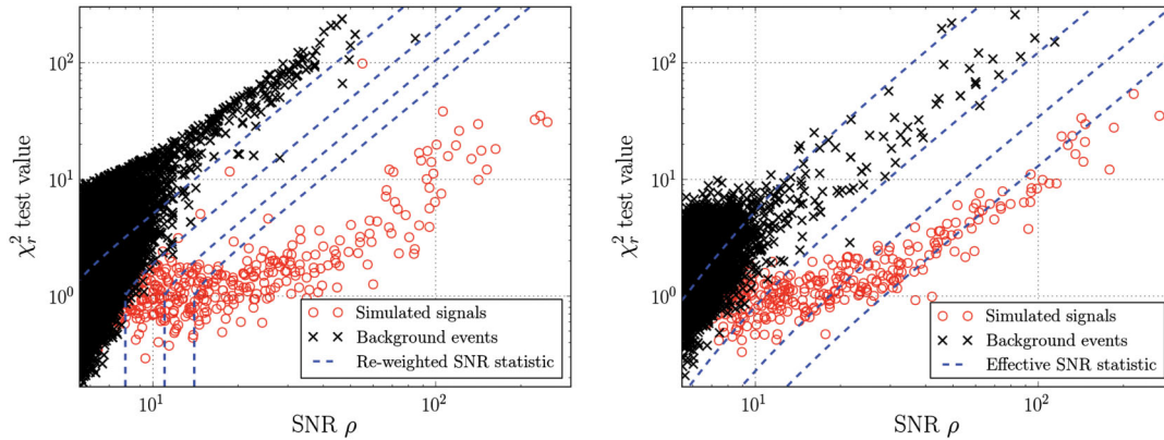
FIG. 2 (color online). Representative distributions of SNR and \chi^2 values for simulated signal (red circles) and background (black crosses) triggers in the LIGO detectors, with contours of the detection statistics used in the search. Note the systematically lower values of \chi^2 for background events with SNR \rho > 10 in shorter-duration templates (right plot) compared to longer-duration (left plot). Left plot—triggers with template duration greater than 0.2 s; dashed lines indicate contours of constant reweighted SNR statistic, Eq. (1). Right panel—triggers with template duration below 0.2 s; dashed lines indicate contours of constant effective SNR, Eq. (2).
