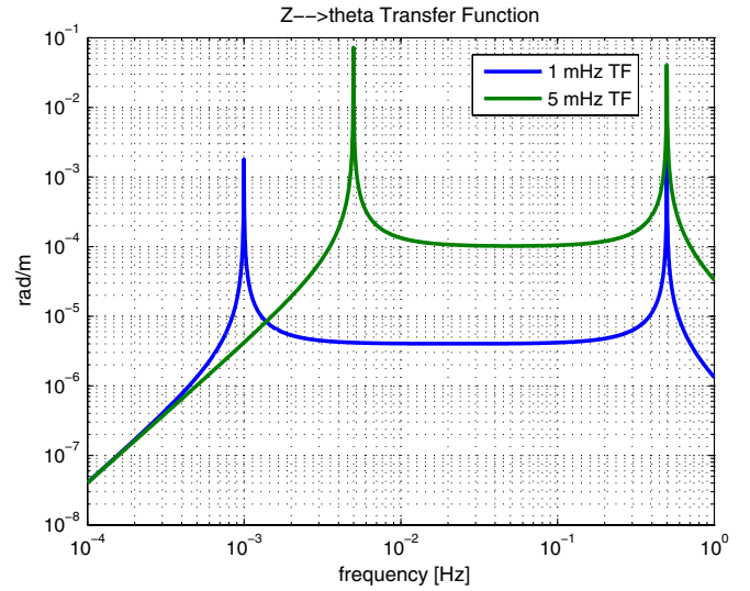
FIG. 6 (color online). Transfer function from the displacement suspension point to the balance's tilt for 1 \text{ mHz} and 5 \text{ mHz} resonance frequency. The coupling depends on the resonant frequency.
