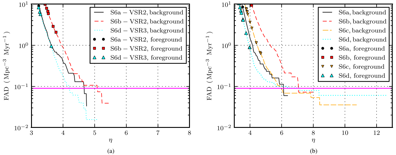
FIG. 1 (color online). (a) H1L1V1 FAD background distributions as a function of \eta and reconstructed events (foreground). (b) H1L1V1 FAD background distributions as a function of \eta and reconstructed events (foreground). The horizontal line denotes the FAD threshold at which the S5-VSR1 and S6-VSR2/3 searches were combined. The threshold was determined by the loudest event identified by the combined S5-VSR1 and S6-VSR2/3 analyses, which had been reconstructed in H1H2L1V1 S5-VSR1 data.
