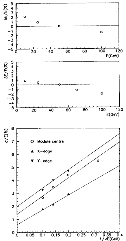
Fig. 2: a) Percentage non-linearity versus energy for a vertical tilt angle of 2.5^\circ (up) and 5^\circ (down). b) Energy resolution as a function of 1/\sqrt{E(\text{GeV})} for the beam hitting the module centre (circles), the x-border (upward triangles), and the y-border (downward triangles). The vertical tilt angle is 2.5^\circ .
