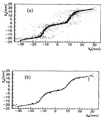
Fig. 3: a) x -coordinate measured by the beam chambers versus the coordinate reconstructed by the calorimeter with a simple 'centre of gravity' algorithm for 50 GeV electrons. b) The same result is shown with superimposed the fit of equation (1).
