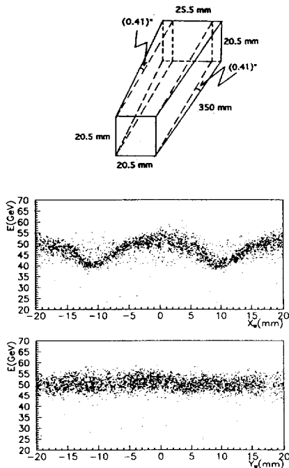
Fig. 1: a) Schematic view of a semiprojective module. b) The calorimeter response uniformity in the horizontal and vertical directions for 50 GeV electrons
