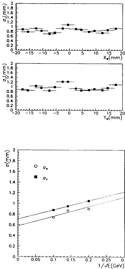
Fig. 5: a) Impact position resolution in x -coordinate and in y -coordinate, as a function of the impact position x and y respectively. The module centre is at about 0 cm, and its edges at -10 cm and 10 cm. The electron energy is 50 GeV. b) Impact point resolution of the electron shower as a function of the electron energy for the horizontal (circles) and the vertical (squares) coordinate respectively. The linear fit in 1/\sqrt{E(\text{GeV})} gives the result quoted in section 2.
