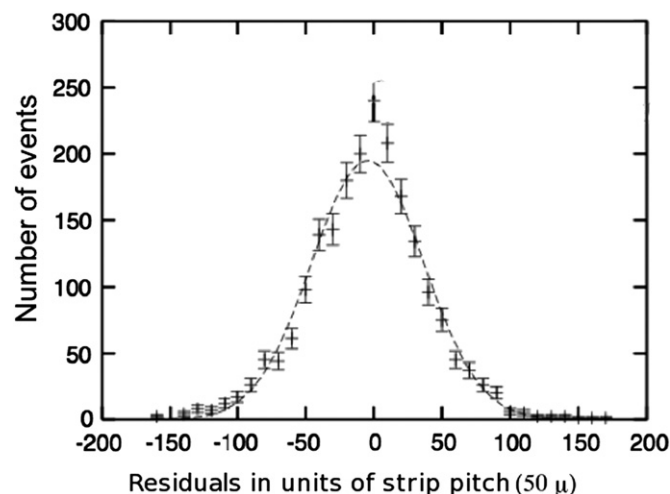
Fig. 7. Spatial resolution obtained with the triangular scintillator bars, as measured with the help of a silicon microstrip tracker. The \sigma is less than 2.5 mm.
