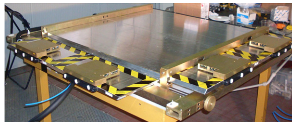
Fig. 13. Fully assembled plane consisting of four basic modules. The external aluminium serves as light shield. The DAQ boards sit on top of each plane in a brass box. Communications are handled through short length LVDS cables.
