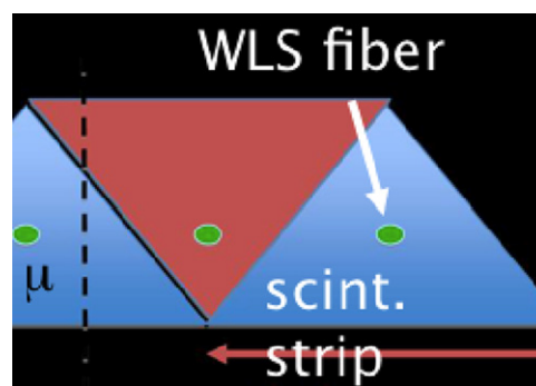
Fig. 4. Thanks to the triangular profile of the scintillators, the muon intersection can be precisely measured as the ratio of light output between two scintillators.
