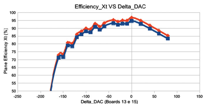
Fig. 14. Efficiency curve for a single plane of the Mu-Ray telescope as a function of SiPM bias (SPIROC DAC). A plateau of 95% is reached.
