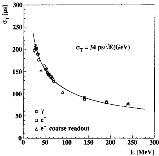
Fig. 4. Time resolution vs. energy.
