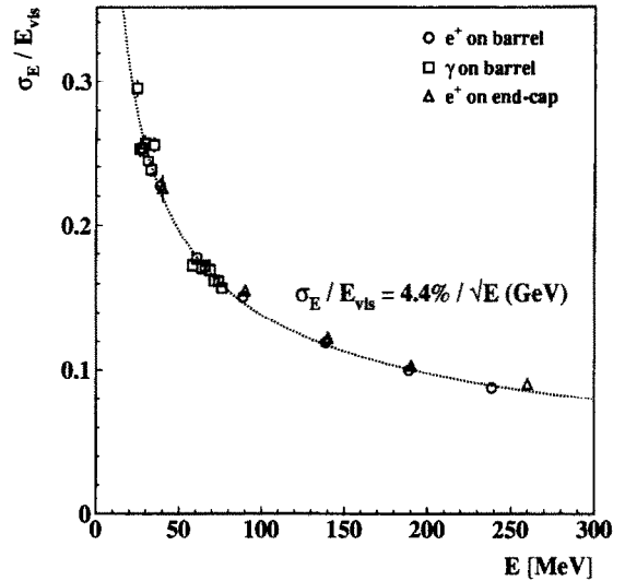
Fig. 3. Energy resolution for photons and positrons vs. kinetic energy.
