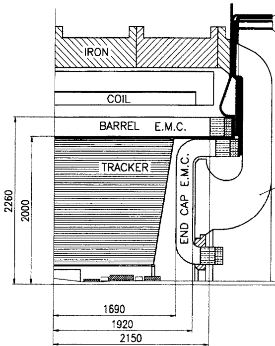
Fig. 1. Cross section of the KLOE calorimeter.
