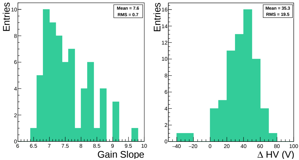
Figure 4. Left: distribution of the HV gain slope (see text for the definition). Right: difference between the determined high voltage values and those provided by the manufacturer to achieve a 3 \times 10^6 gain.
