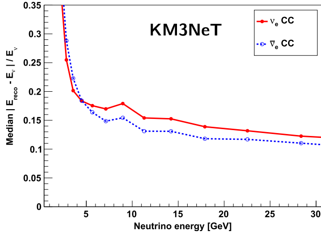
Figure 86. Median fractional energy resolution ( |E_{\text{reco}} - E_{\nu}| / E_{\nu} ) as a function of neutrino energy for \nu_e CC (red) and \bar{\nu}_e CC (blue) events weighted according to the Bartol flux model.
