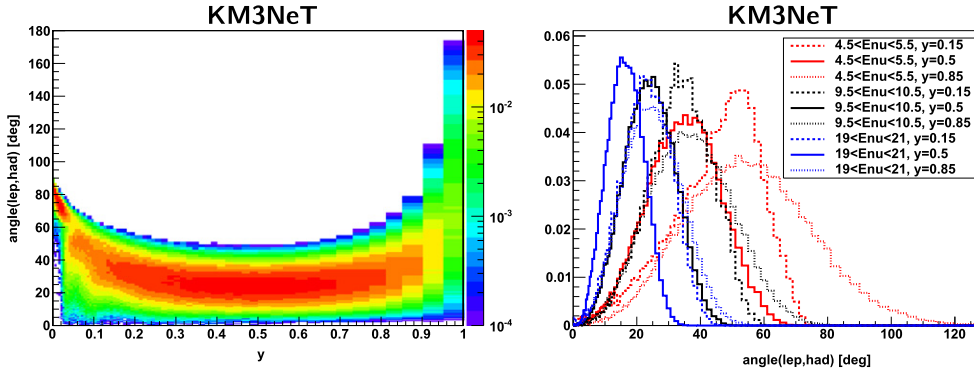
Figure 66. Angle between the outgoing muon and the outgoing hadronic shower \phi_{\text{lep,had}} from \nu_\mu CC interactions with 9.5 < E_\nu/\text{GeV} < 10.5 as a function of inelasticity y . The kinematics looks very similar for \nu_e CC interactions. The features at 0 < y < 0.2 are due to the different neutrino interaction channels (see figure 57). Each column of bins in y is normalised to 1 (left). Distribution of the opening angle \phi_{\text{lep,had}} in \nu_\mu CC interactions for three different inelasticities y and neutrino energies (right).
