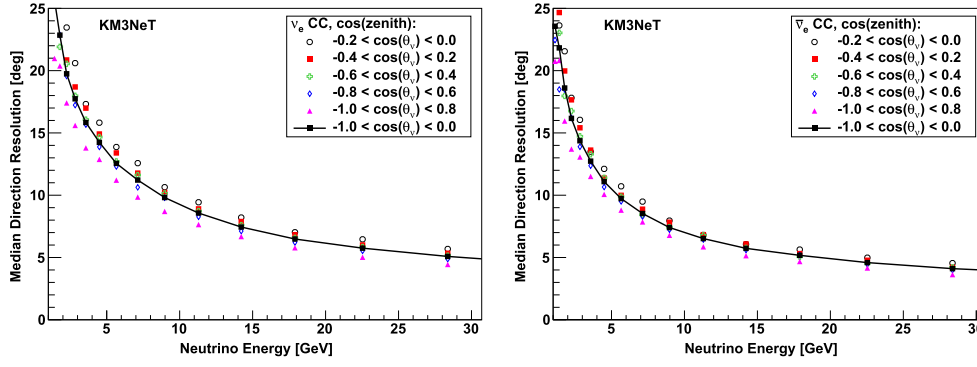
Figure 80. Median neutrino direction resolution (angle between reconstructed direction and neutrino direction) as a function of neutrino energy for different true neutrino \cos(\text{zenith}) ranges, where \cos(\text{zenith}) = -1 means vertical up-going and \cos(\text{zenith}) = 0 means horizontal. The black line corresponds to up-going neutrinos weighted according to the Bartol flux model. \nu_e CC (left) and \bar{\nu}_e CC (right).
