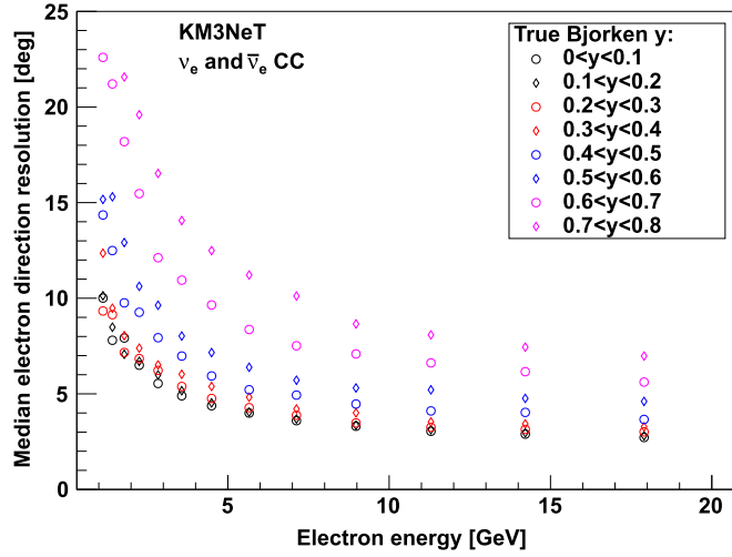
Figure 82. Median electron direction resolution (angle between reconstructed direction and electron direction) as a function of electron energy for up-going \nu_e and \bar{\nu}_e CC events weighted according to the Bartol flux model. Different marker colours and styles represent different true inelasticity y ranges.
