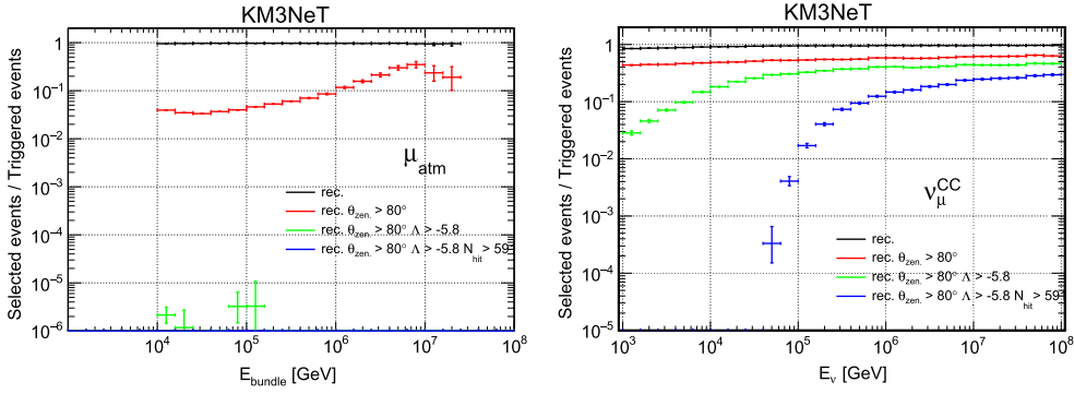
Figure 32. Ratio of the numbers of selected events and triggered events at each step of the track analysis (see text) for atmospheric muons (left) and \nu_\mu CC neutrino reactions (right) as a function of the primary energy.
