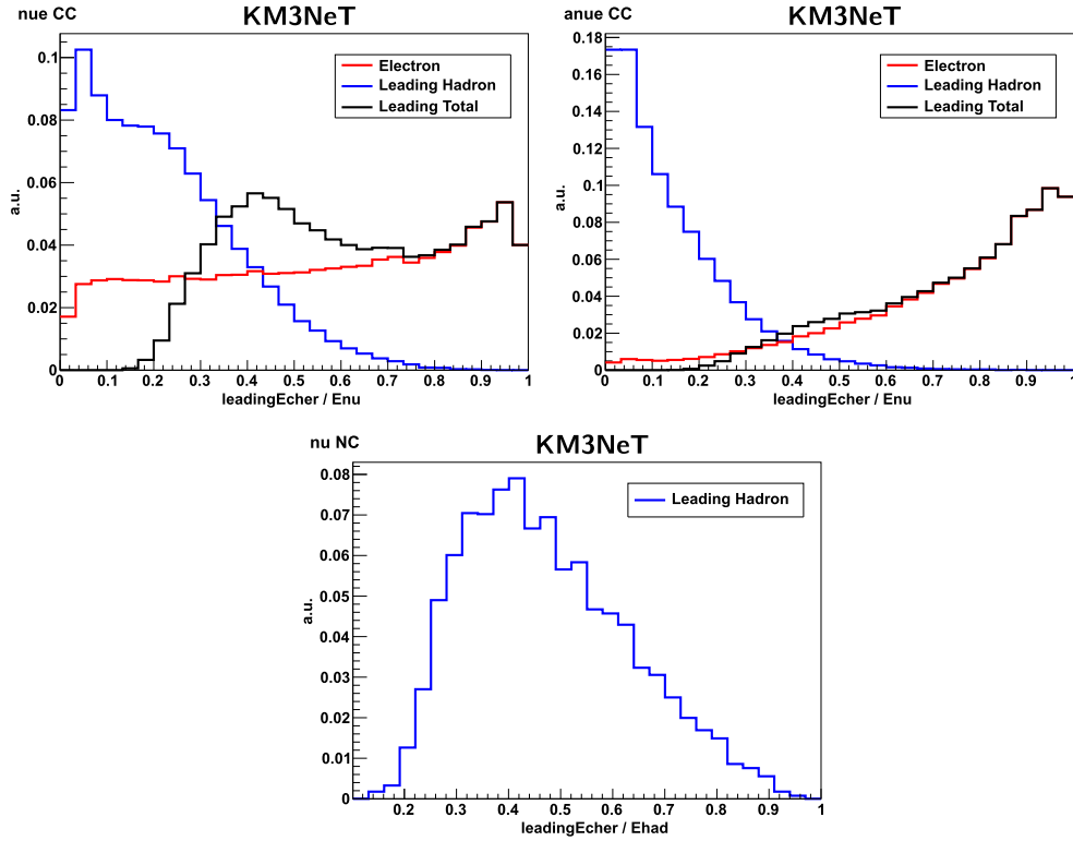
Figure 73. Distribution of E_e/E_\nu (red), the leading E_{had}^{cher}/E_\nu in the hadronic shower (blue) and the leading E_{tot}^{cher}/E_\nu of the total event (black). Top left: \nu_e CC events with 9 \text{ GeV} < E_\nu < 11 \text{ GeV} . Top right: \bar{\nu}_e CC events with 9 \text{ GeV} < E_\nu < 11 \text{ GeV} . Bottom: \nu_e and \bar{\nu}_e NC events with 9 \text{ GeV} < E_{had} < 11 \text{ GeV} .
