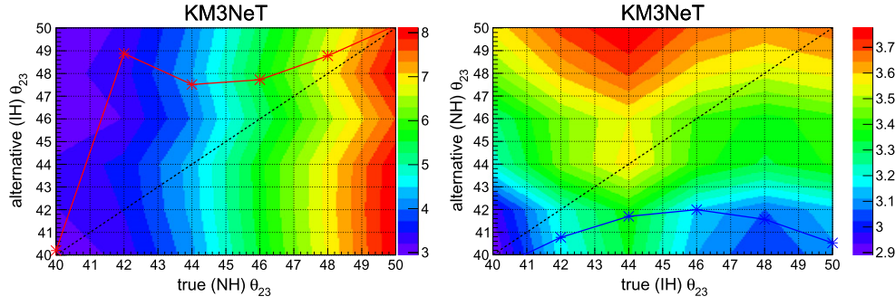
Figure 104. The mass hierarchy sensitivity for the true normal (left) and inverted (right) hierarchy. The horizontal axis indicates the true value of \theta_{23} . The vertical axis indicates the ‘alternative’ value of \theta_{23} : the value belonging to the hypothesis that is being rejected. The diagonal dashed lines indicate the position where the alternative \theta_{23} is the same as the true one. Along these lines the mass hierarchy sensitivity according to the original method can be read off. The solid red and blue lines show the most likely alternative value for each true \theta_{23} . They are the most likely value when fitting \theta_{23} under the wrong hierarchy assumption. Along these lines the mass hierarchy sensitivity according to the new method can be read off.
