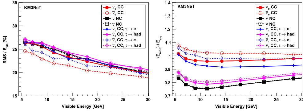
Figure 87. Relative energy resolution \text{RMS}/E_{\text{vis}} as a function of the visible energy E_{\text{vis}} for shower-like neutrino interaction channels (left) and mean relative offset in reconstructed energy— given as \langle E_{\text{reco}} \rangle / E_{\text{vis}} —as a function of E_{\text{vis}} (right).
