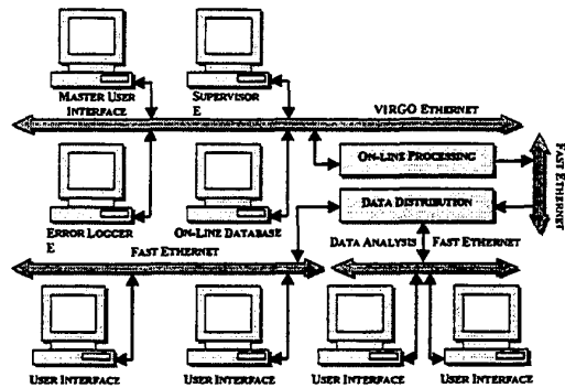
Fig.5: Client/Server architecture of the Virgo Data Distribution System
