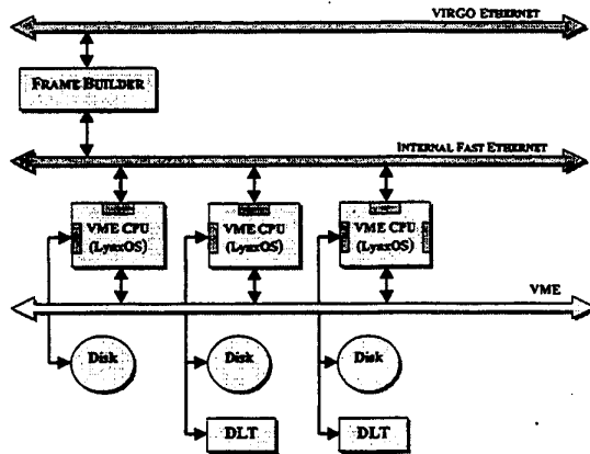
Fig.3: Architecture of the Virgo Raw Data Archiving Server
