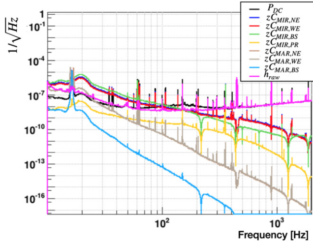
Figure 12. Contributions of the mirrors longitudinal controls to the reconstructed signal h_{\text{raw}} in O. Black curve is the amplitude spectral density of the dark fringe signal P_{\text{DC}} . Pink curve is the amplitude spectral density of h_{\text{raw}} purple in watt units. The other curves are the contribution of the various controls zC_i in the same units.
