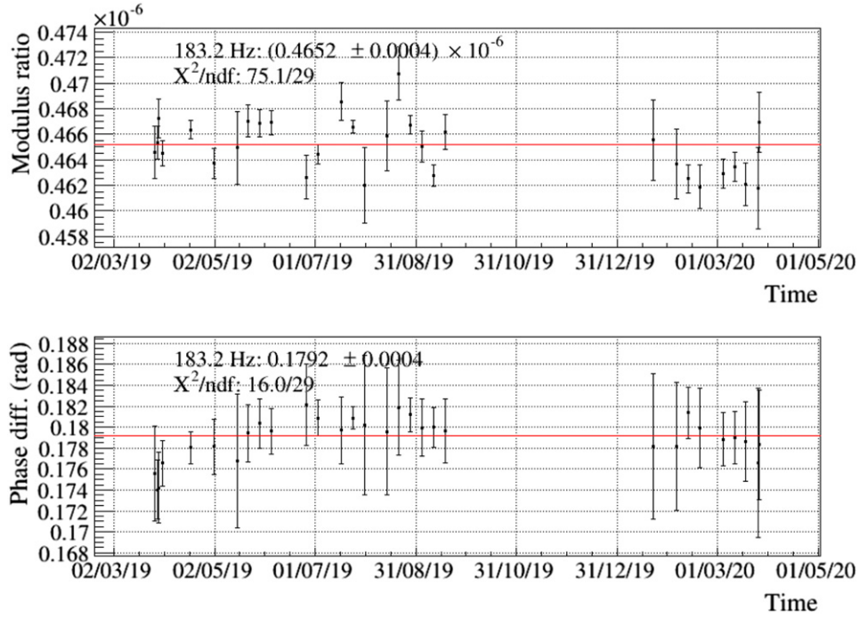
Figure 2. Evolution of the NE TF ratio used to transfer PCal to EM actuator calibration as a function of time at 183.2 Hz during O3 (see equation (9)). The NE PCal laser could not be used from October 2019 to mid-January 2020. The laser was replaced and the PCal photodiodes re-calibrated mid-January 2020.
