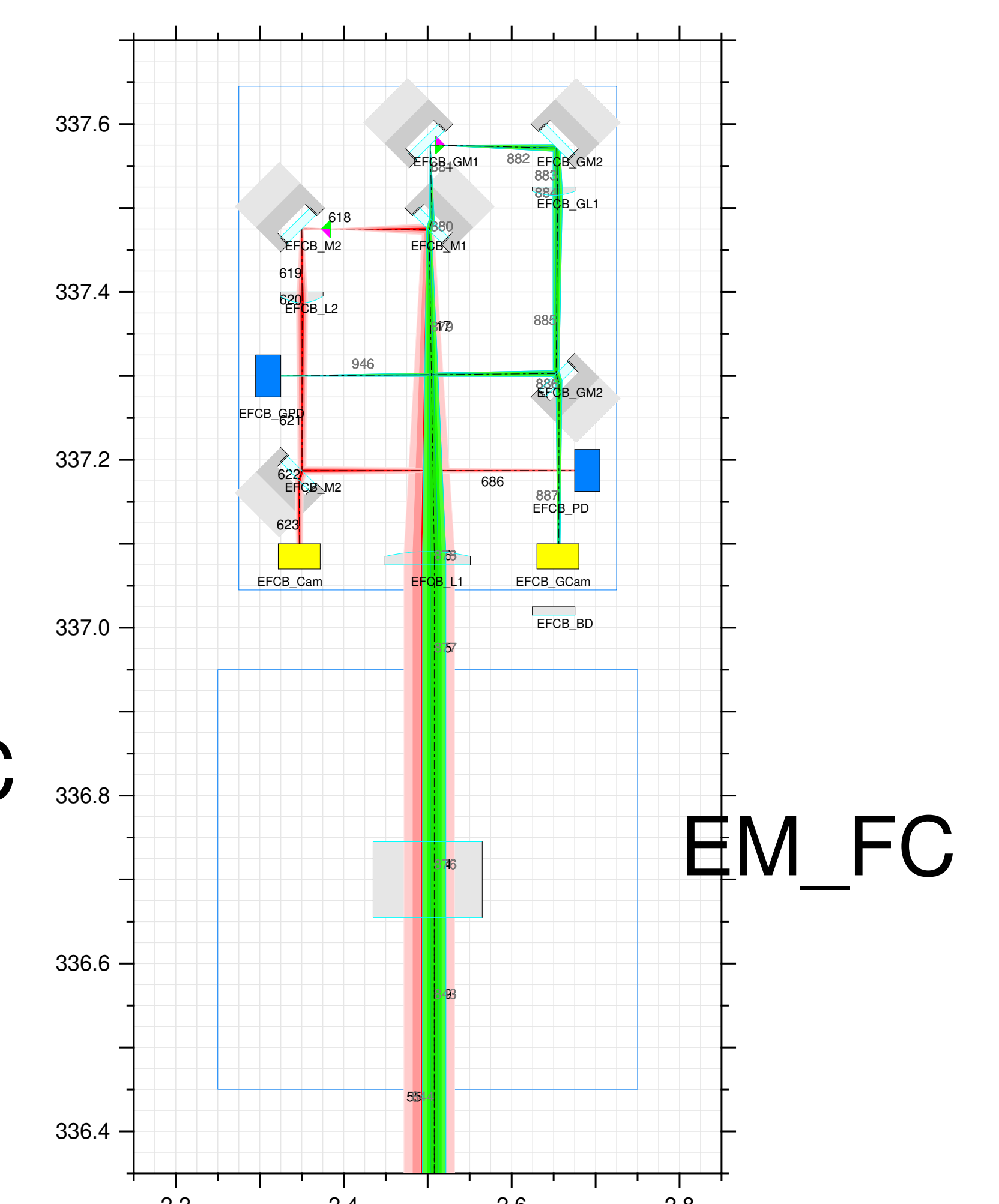
End Mirror Filter Cavity (EMFC)
