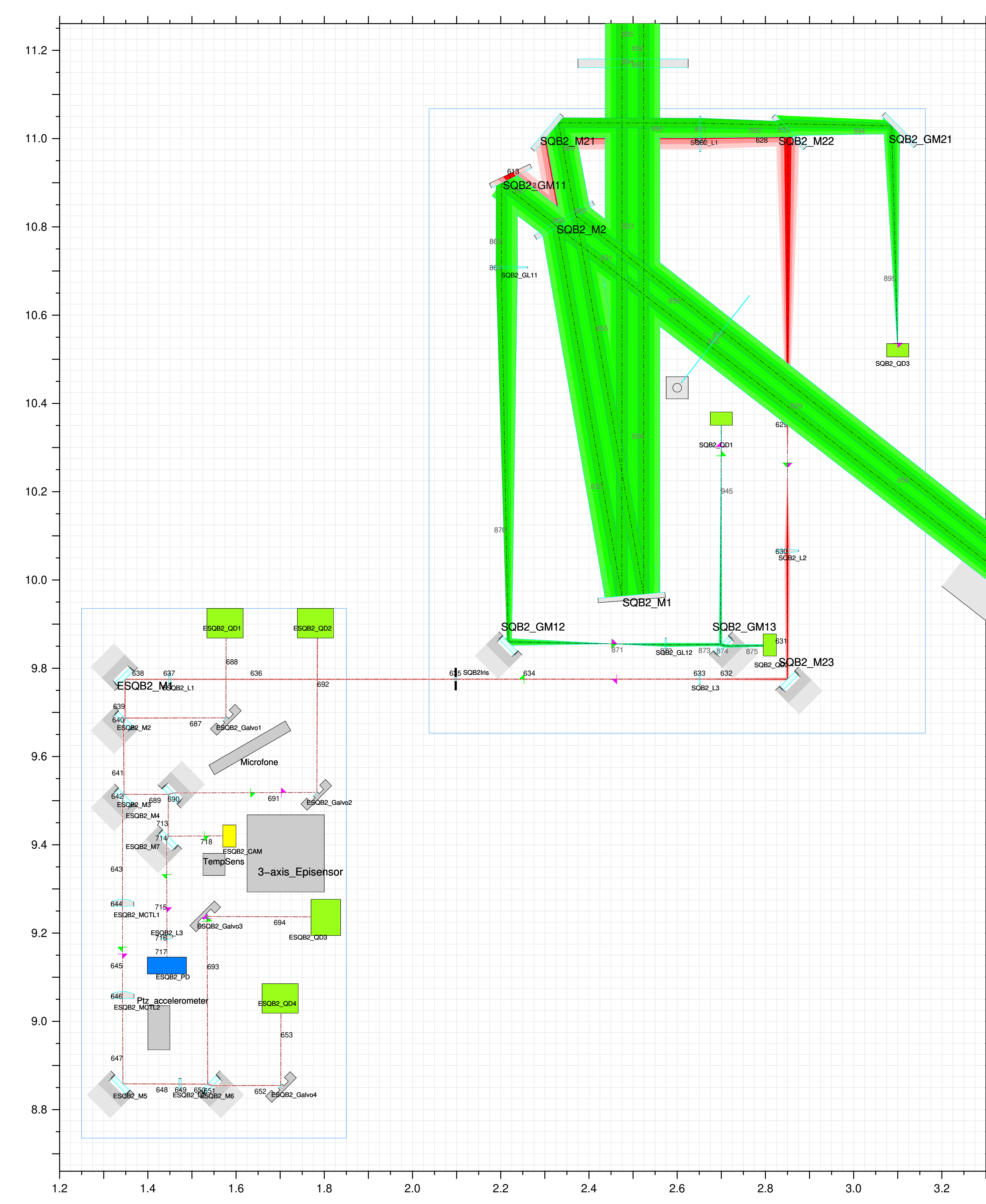
Suspended sQueezing Bench 2 (SQB2) & ESQB2
