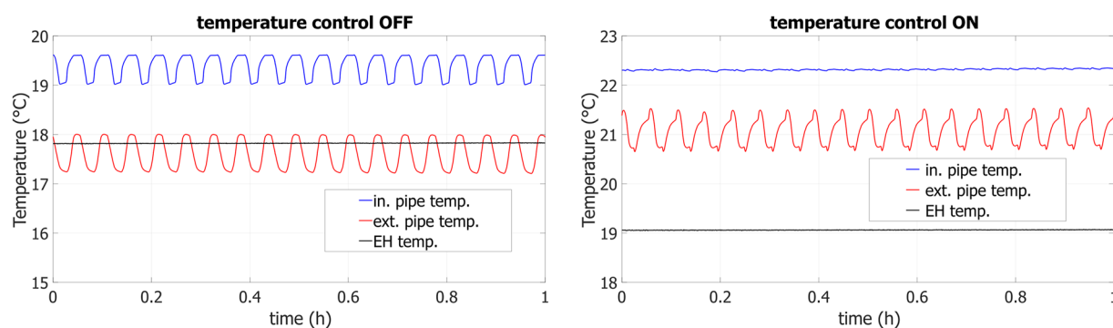
FIG. 11. Measured OLP (red) and ILP (blue) temperatures without (left) and with (right) temperature control. When the loop is closed, the ILP temperature excursion is greatly reduced. The black line shows the temperature of the EH, which is insensitive to the changes in the ILP temperature.
