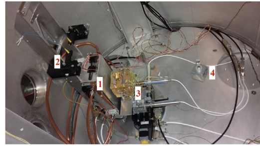
FIG. 2. The LAG apparatus in the vacuum chamber, seen from above. 1—Field mass container; 2—optical readout for the FM; 3—electrode housing, surrounding the test mass with sensing and control electrodes; and 4—counterweight mass for balancing.
