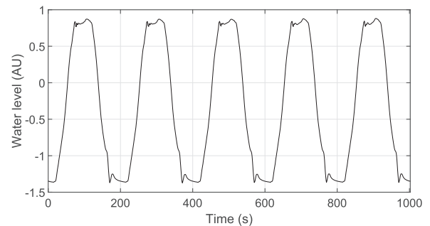
FIG. 5. Liquid level time evolution as measured by the optical lever sensor. The tank is filled and emptied with a period T_m = 1/f_m = 200 s.
