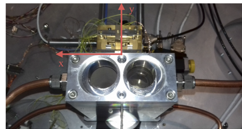
FIG. 3. The field mass containers as viewed from above. The copper tubes for the liquid circulation are visible on the background, while those in the foreground connect to the compensation mass container, outside the vacuum chamber, to keep the vapor pressure constant. The test mass is inside the gold-plated electrode housing: they can be moved together along both the x and y horizontal axes, shown superimposed on the picture.
