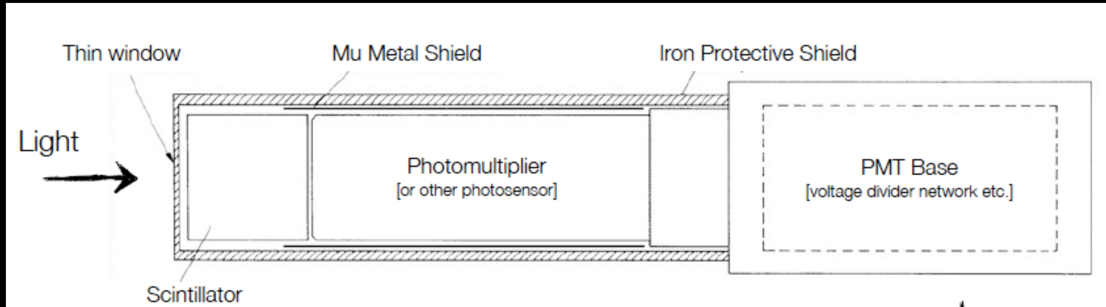
SCHEME OF A SCINTILLATION + PMT DETECTOR
