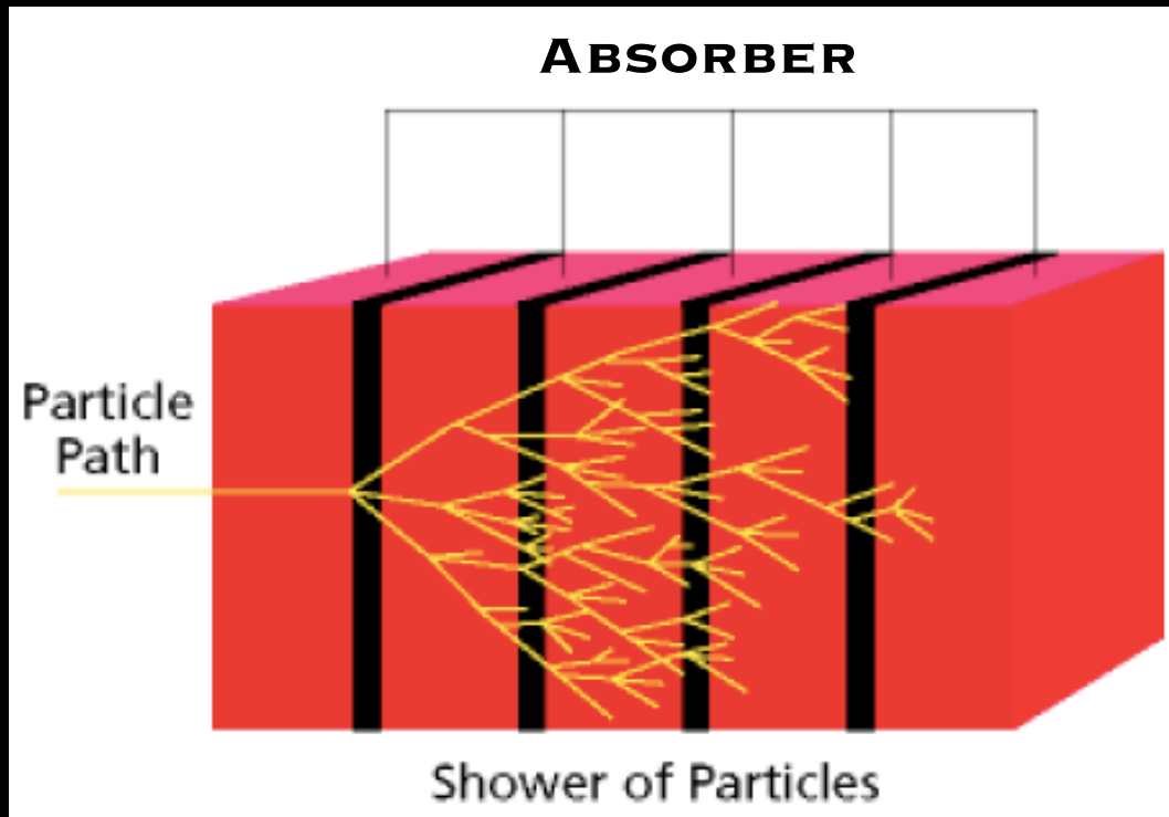
SCHEME OF A CALORIMETER
