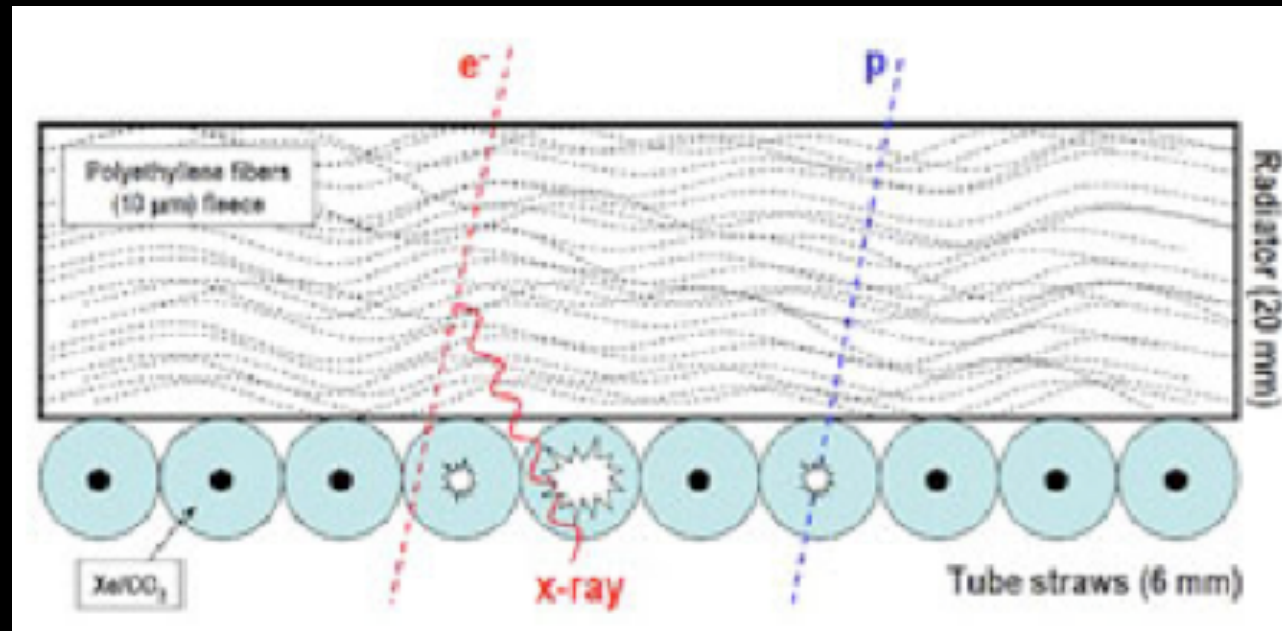
PRINCIPLE OF DETECTION OF TRANSITION RADIATION DETECTORS
