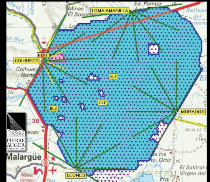
AUGER DETECTOR (60X60 KM)
