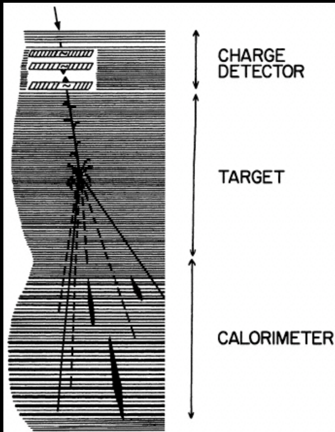
SCHEME OF JACEE
