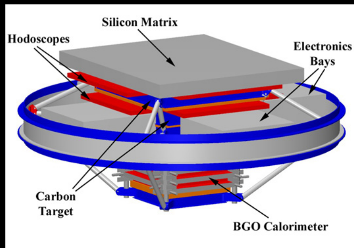
ATIC DETECTOR (60X60 CM)
