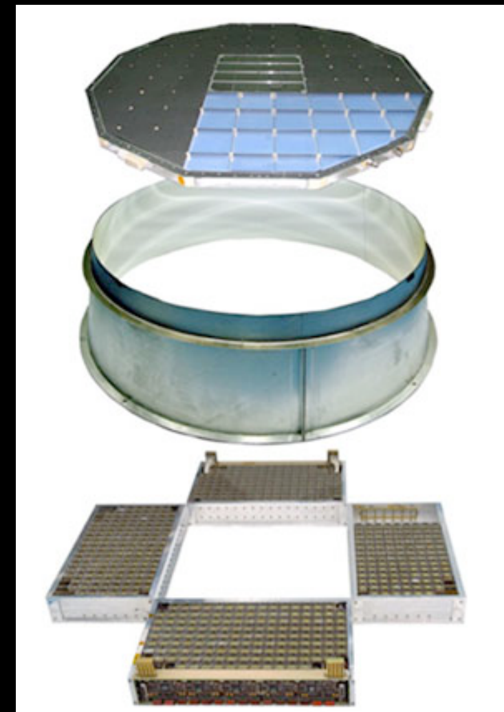
AMS CHERENKOV DETECTOR: RADIATOR, MIRROR, PMTs
