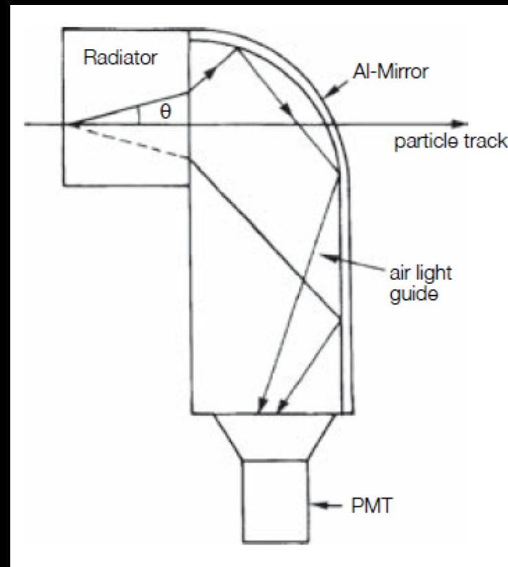
WORKING PRINCIPLE OF A CHERENKOV DETECTOR
