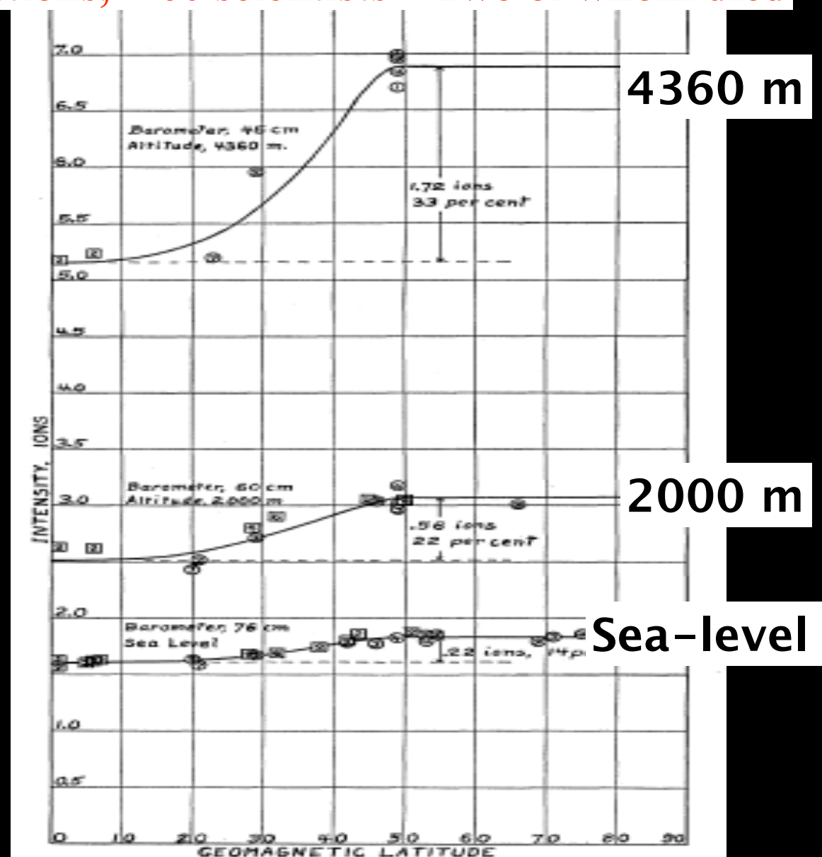
FIG. 6. Intensity vs. geomagnetic latitude for different elevations.
