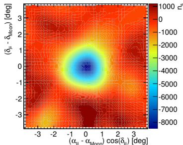
Moon Shadow in Cosmic Ray Muons in IceCube (59 strings)
