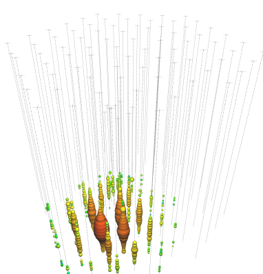
71.5 TeV, -60^\circ
