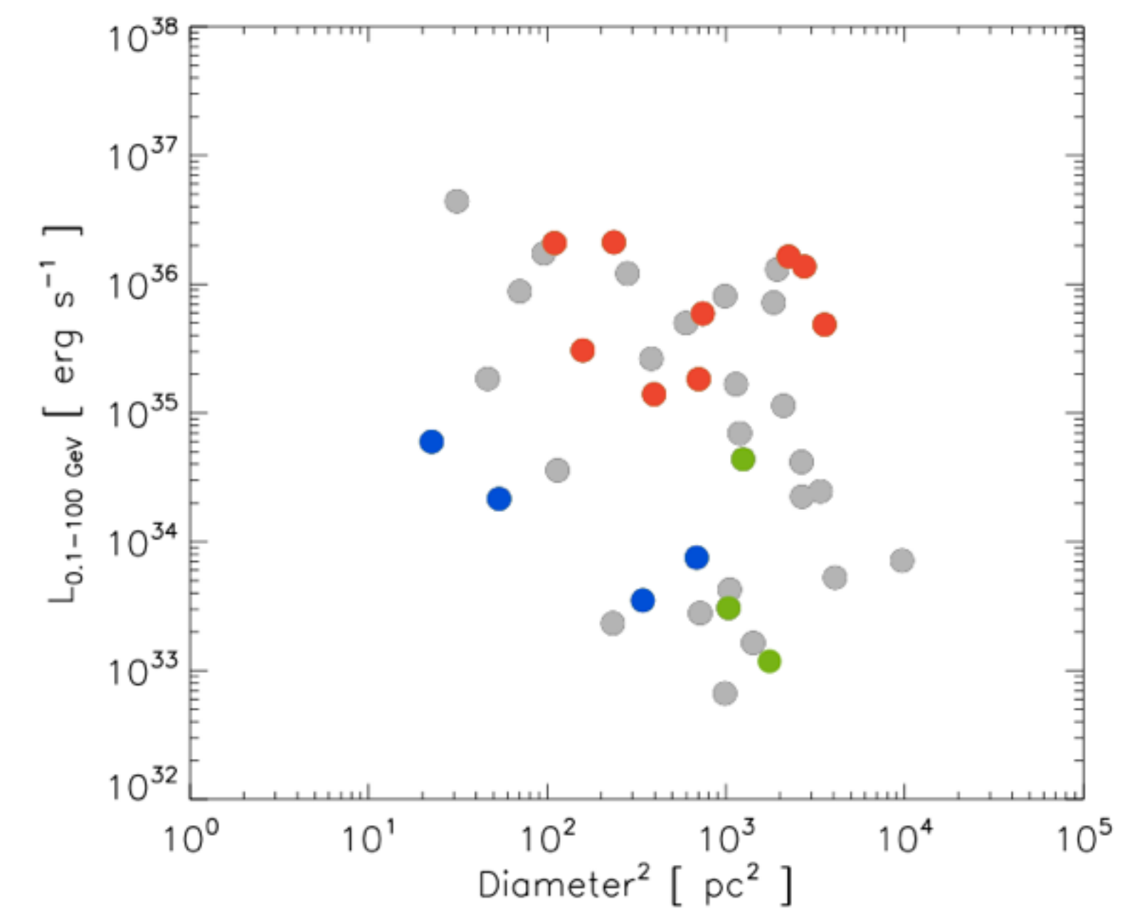
Figure 3. Gamma-ray luminosity plotted as a function of diameter squared (using the radio size). Among identified SNRs, those interacting with molecular clouds are brighter than young SNRs and those evolving in the diffuse ISM.
