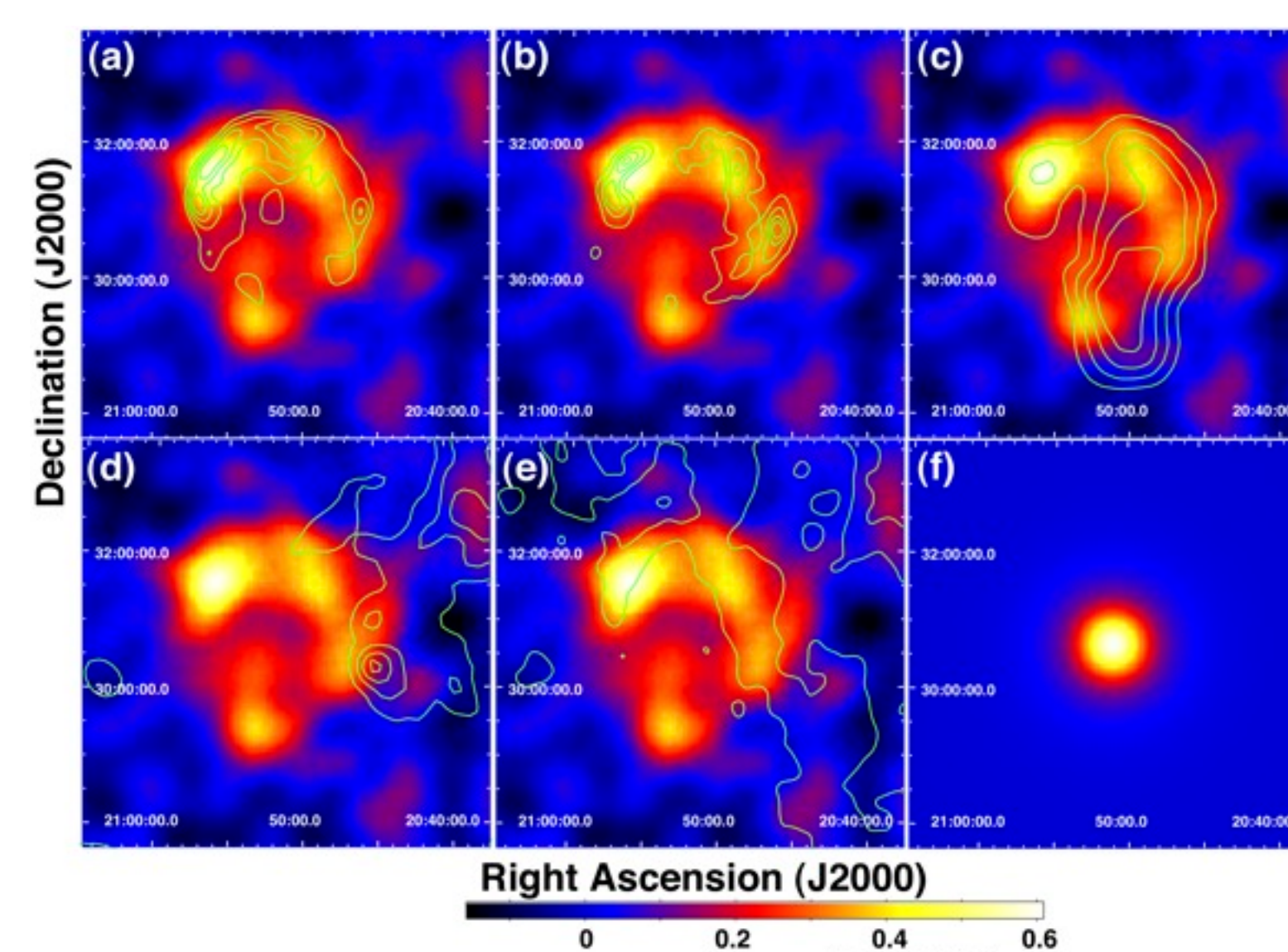
Figure 4. Background-subtracted counts maps at 0.5-10 GeV [8]. Contours correspond to images of: (a) X-rays, (b) H \alpha , (c) Radio, (d) CO, (e) HI, (f) the LAT PSF.
