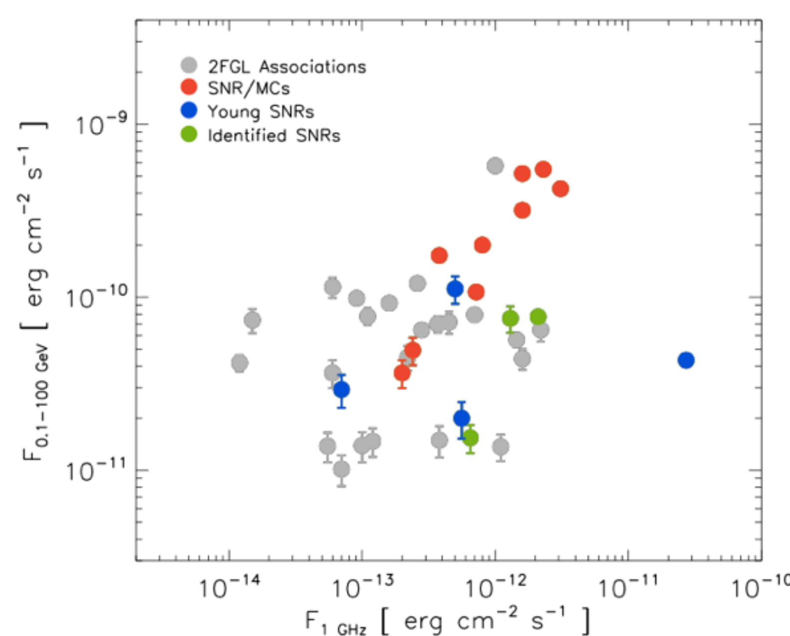
Figure 2. Synchrotron radio (1GHz) flux vs. gamma-ray (0.1-100 GeV) flux. Large scatter is seen for all 2FGL-detected SNRs, however a correlation can be seen for the subset of identified SNRs known to be interacting with molecular clouds.
