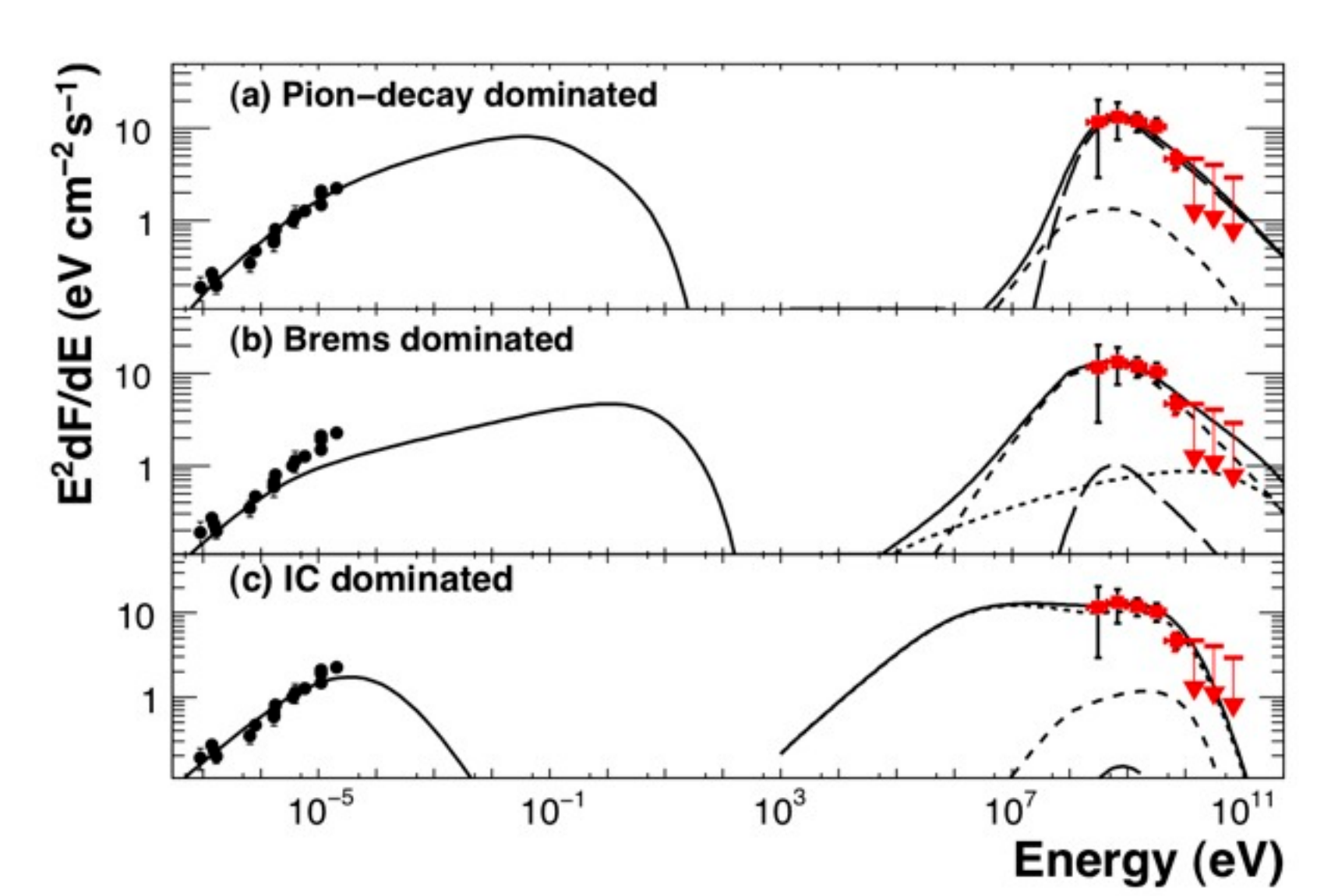
Figure 5. Multi-band spectral fits to radio and gamma-ray emission [8]. All models show different combinations of \pi^0 decay (long-dash), bremsstrahlung (dash), and IC (dotted).
