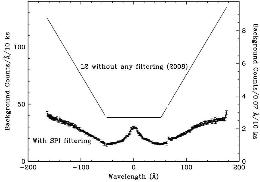
Figure 9.22: The Jan 2008 LETG+HRC-S background rate with and without pulse-height filtering. These Level 2 rates correspond to 1.1 \times 10^{-6} cts s ^{-1} pixel ^{-1} (see Figure 9.21). Data are shown using the standard ‘bowtie’ spectral extraction region (see Figure 9.14). X-ray losses from the observed spectrum as a result of the filtering for 1st order are \sim 1.25\% ; losses will be slightly higher for higher orders. See http://cxc.harvard.edu/cal/Letg/Hrc_bg for more information.
