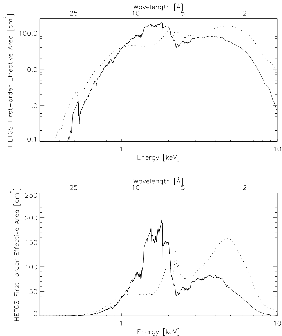
Figure 8.11: The modelled total first-order (solid curve) and zeroth-order (dotted curve) effective area, integrated over the PSF, of the HRMA -HETG-ACIS-S combination, as a function of energy. The first-order data are the same as those plotted in Figures 8.7 and 8.9. The plotted first-order values are the sums of the area at a particular energy from both orders (+/-) of both MEG and HEG spectra. Both a log-log and a log-linear version are shown.
