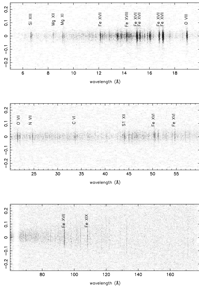
Figure 9.25: HRC-S detector image of a Capella observation, showing positive order dispersion. Both axes are in \text{\AA} with 1.148 \text{ \AA/mm} . The increasing cross-dispersion extent of lines at longer wavelengths is due to astigmatism in the HRMA/LETG system. The positive-order HRC-S plate gap is at \sim 63 \text{ \AA} .
