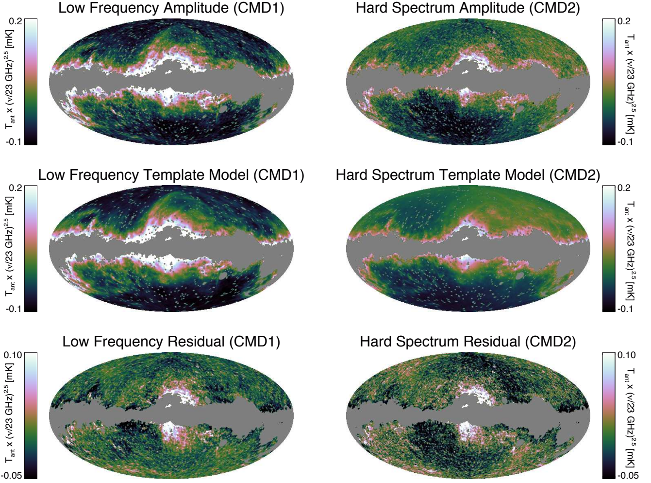
Fig. 3. Left column, top: The recovered amplitude of the low-frequency component at 23 GHz from our simplest Commander fit to the Planck data alone, CMD1. As shown in Pietrobon et al. (2012) , while this model provides an excellent description of the data, this low-frequency component is actually a combination of free-free, spinning dust, and synchrotron emission ( top ). Left column, middle: a four-component template model of this component (see Table 2). Left column, bottom: The haze residual. The residuals are small outside the haze region indicating that the templates are a reasonable morphological representation of the different components contained in the Commander solution. The haze residual is strikingly similar to that found for the template-only approach in Fig. 2 (though there does seem to be a residual dipole in the Commander solution). Right column: The same, but for the CMD2 low-frequency, hard spectrum component. While there is still some leakage of dust-correlated emission in the solution, the softer synchrotron emission (mostly correlated with the 408 MHz template [see Fig. 6]) has been separated by Commander. The resultant map is dominated by free-free and the haze emission and the regressed haze residual ( bottom panel ) shows morphology very similar to both the template fitting and CMD1 results indicating that the haze has been effectively isolated.
