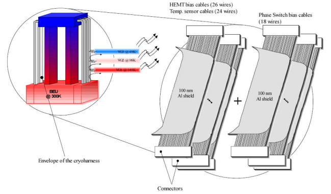
Fig. 23. Schematic of the cryoharness serving HEMT biasing, phase switch biasing and temperature sensors. Heat loads on the 20 K stage are minimised by intercepting heat with the V-grooves.
