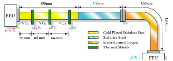
Fig. 17. Schematic of the LFI composite waveguide design, showing representative dimensions of the various sections as described in the text.
