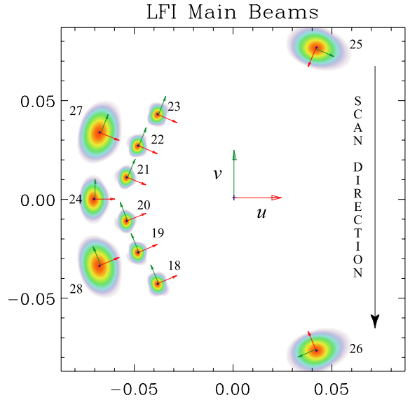
Fig. 11. Footprint of the LFI main beams on the sky and polarization angles as seen by an observer looking towards the satellite along its optical axis ( (u, v) plane (see Sandri et al. (2009) for details). Labels from 18 to 23 refer to 70 GHz horns, from 24 to 26 refer to 44 GHz horns, and 27 and 28 refer to 30GHz horns. The scan direction, orthogonal to the focal plane symmetry axis, is indicated by an arrow. All the relative angles in pairs of feeds aligned along the scan direction are shifted by 45^\circ , with the exception of RCA24.
