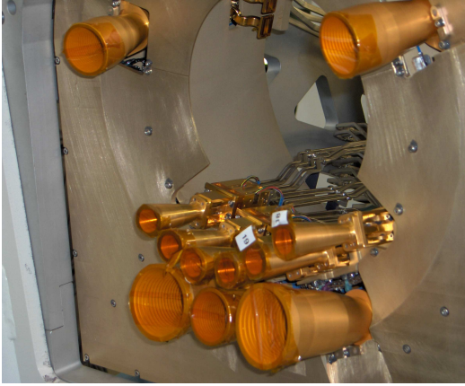
Fig. 10. Arrangement of the LFI feeds in the focal plane. Top: mechanical drawing of the main frame and focal plane elements. Shown are the bipods connecting the FPU to the telescope structure. Bottom: picture of the LFI flight model focal plane.
