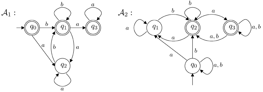
Fig. 4. NBWs for a^* \cdot b \cdot (a + b)^* .
