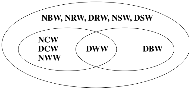
Fig. 1. The expressiveness hierarchy for \omega -regular automata.
