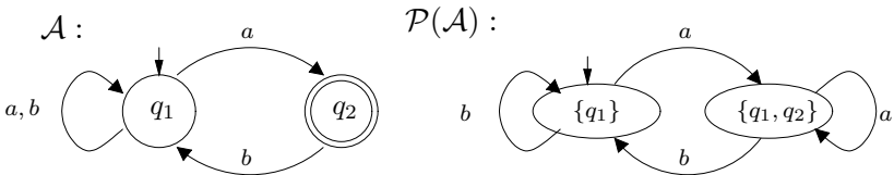
Fig. 6. An NBW for ((a + b)^* \cdot a \cdot b)^\omega that is not Büchi-powerset-type.
