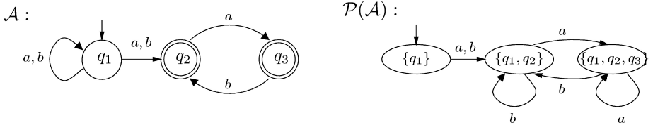
Fig. 7. An NBW for (a + b)^* \cdot (a \cdot b)^\omega that is neither co-Büchi-, Rabin-, nor Streett-powerset-type.
