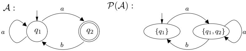
Fig. 8. An NBW for (a^+ \cdot b)^\omega that is powerset-type but not finite-type.
