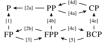
Figure 7: Implication Schema.
