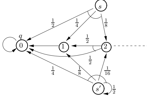
Figure 4: An infinite Markov chain in which states s and s' cannot be distinguished by \text{QRCTL}^{>0} , but are distinguished by the ATL formula \langle\langle p \rangle\rangle \square \neg q .
