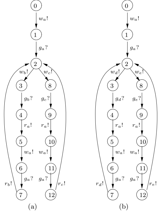
Figure 6: Thread interfaces from Example 2.
