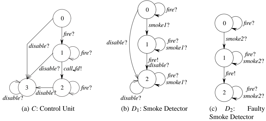
Fig. 1. Sociable interface automata for a fire detection system.
