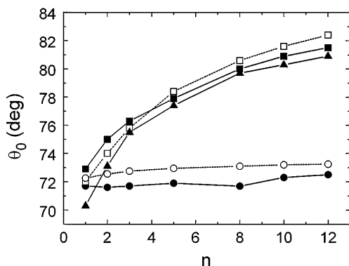
FIG. 1. Average polar angle \theta_0 of n CB molecules vs alkyl chain length n obtained by SHG measurement (solid symbols) and by theoretical calculations (open symbols). Squares, triangles, and circles refer to P6 substrates, fused silica substrates, and air-water interface, respectively.
