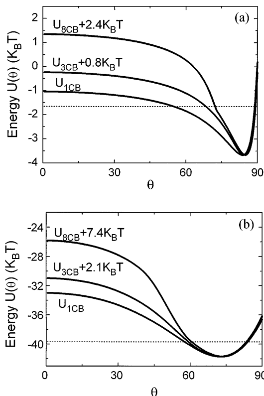
FIG. 3. Potential energy U experienced by an n CB molecule as a function of its polar angle \theta . Only three representative cases, n = 1, 3 , and 8 , are shown. Dotted line is at 2k_B T above the minimum of the potential wells. (a) On solid substrates and (b) at air-water interface.
