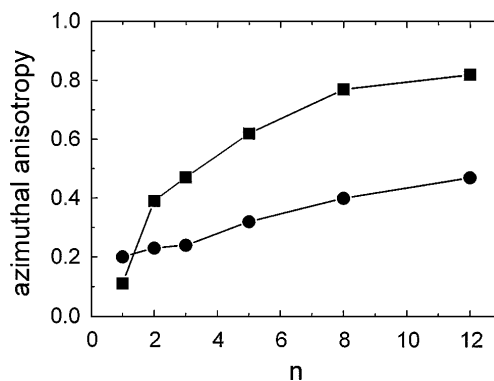
FIG. 2. Measured azimuthal anisotropic parameters d_1 and d_2 of n CB molecules on rubbed P6 vs alkyl chain length n . Circles are for d_1 and squares are for d_2 .
