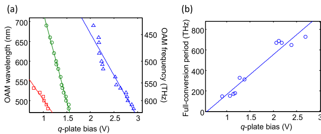
Fig. 3. (a) OAM full-conversion wavelength (and frequency) as a function of the q -plate bias; (b) full-conversion period in frequency as a function of the q -plate bias.
