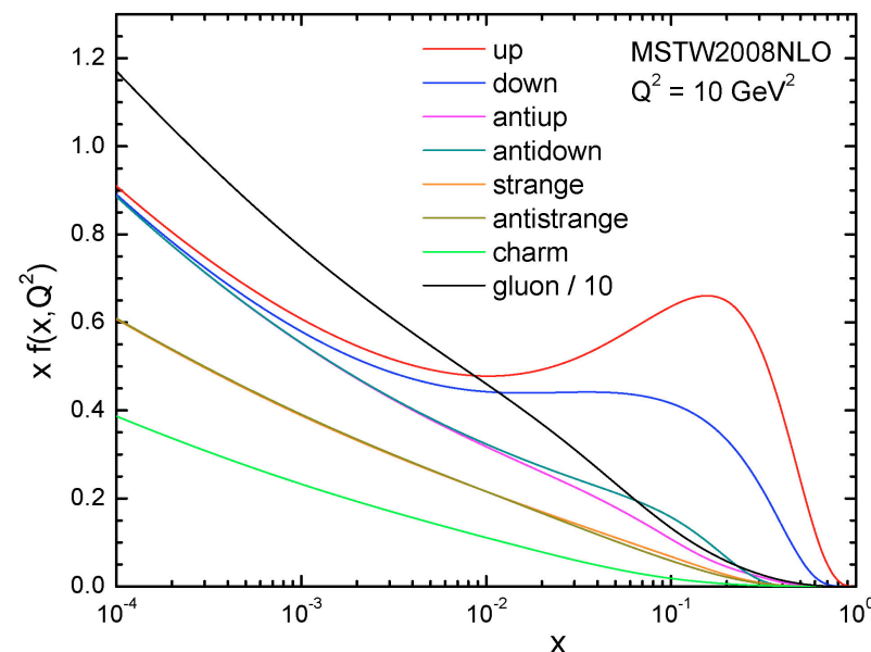
Parton Distribution Functions
