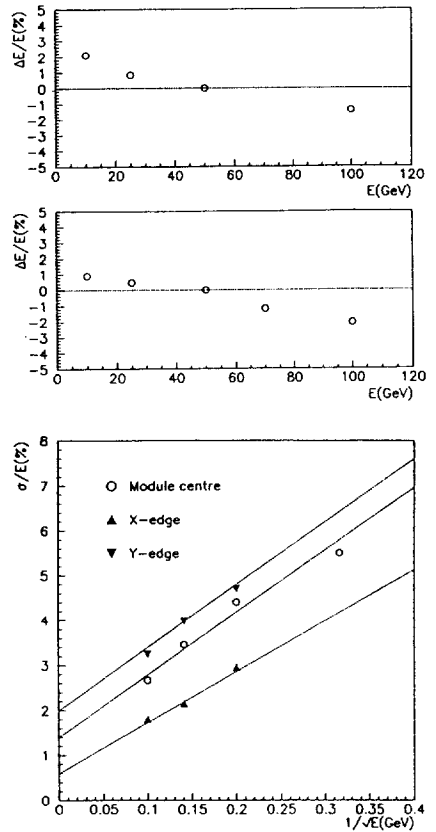
Fig. 2: a) Percentage non-linearity versus energy for a vertical tilt angle of 2.5° (up) and 5° (down). b) Energy resolution as a function of 1/\sqrt{E(\text{GeV})} for the beam hitting the module centre (circles), the x-border (upward triangles), and the y-border (downward triangles). The vertical tilt angle is 2.5°.
